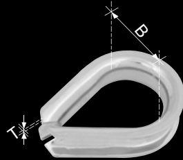
Metric SF234U Light thimbles
