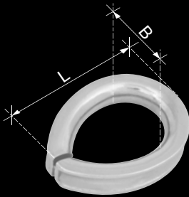
Metric S2343 Opened end thimbles
